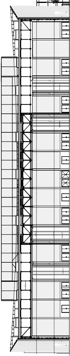
Snitt øst Cross section east
